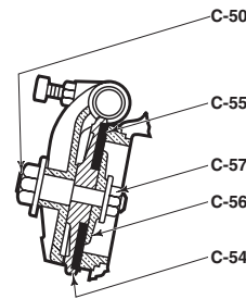
Rubber faced disc and clapper 3"-12"
