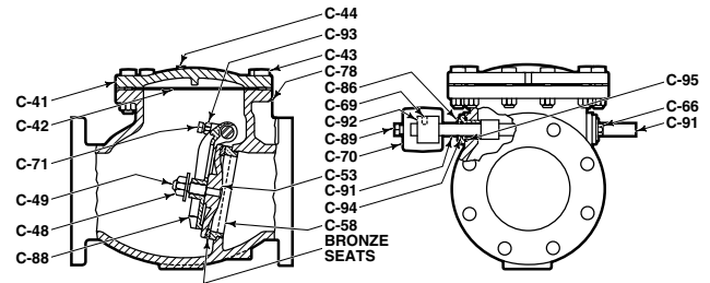
Valve body and clapper 3"-12" Metal faced disc shown
