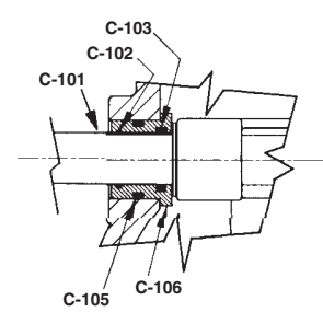
Hinge pin and stuffing box†† 4"-12"
