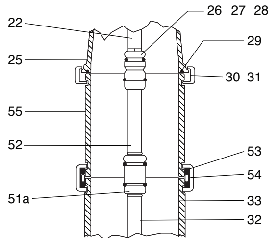
DETAIL OF EXTENSION SECTION
