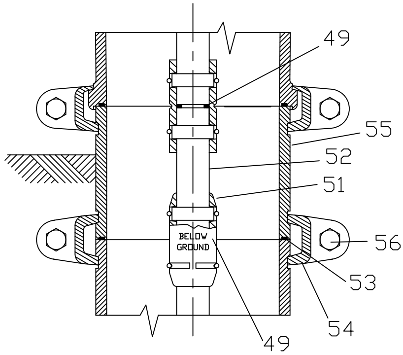
DETAIL OF HYDRANT EXTENSION
